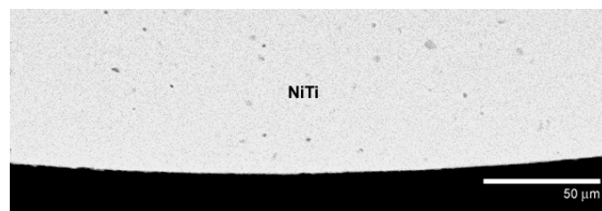
Figure 4: BEI image of as-electropolished cross-section (500X)
